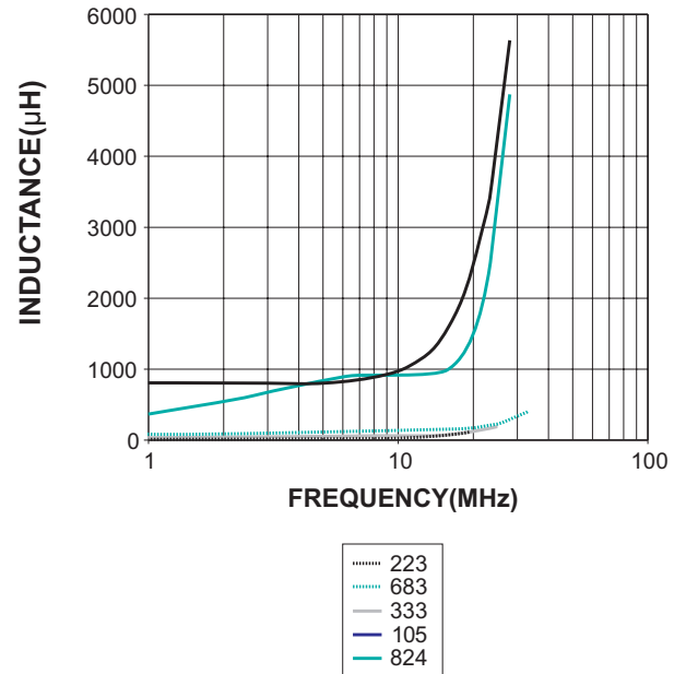
Typical Inductance vs Frequency
