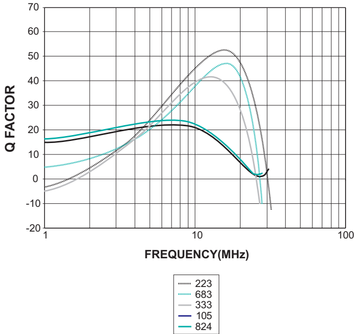
Typical Q vs Frequency
